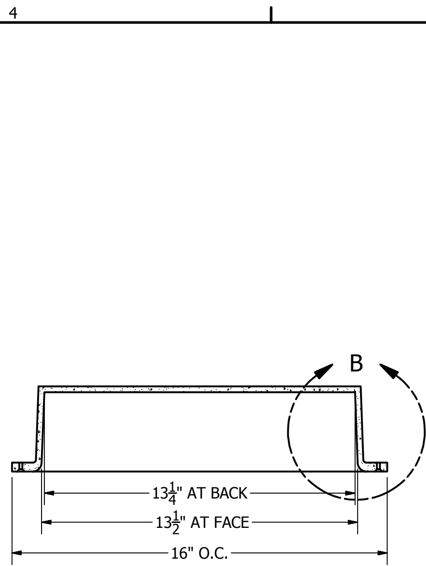
SECTION A-A SCALE 1 / 4
